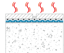
Heating Distribution
